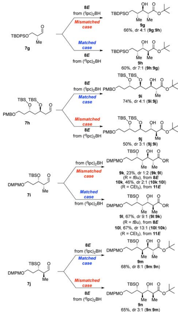
Scheme 5. Double Asymmetric Aldol Reactions of Chiral Aldehydes and the Chiral E -Enolborinate Generated from 4a,b a-d
